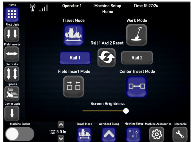
Operator Touchscreen Control Panel for Workhead Adjustment and Diagnostic Troubleshooting
